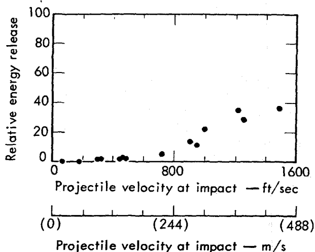
Fig 4 Susan Test: Comp B-3. Conversion factor: 1 ft/sec = 3.048 \times 10^{-1} m/s
